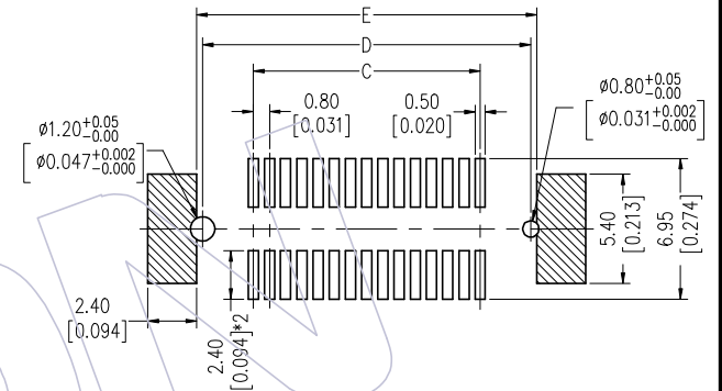
Recommended P.C.B Layout(Top Side) (PCB BOARD TOLERANCE±0.05)
