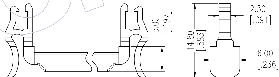
BUTTERFL Strain Relief P/N: G5210-XXDX02
