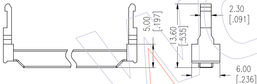
Strain Relief P/N: G5210-XXDX01
