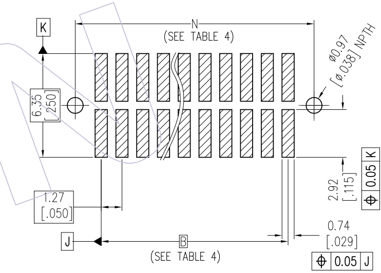
Recommended P.C.B Layout(Top Side) (PCB BOARD TOLERANCE±0.05)
