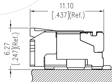
ASSEMBLY
