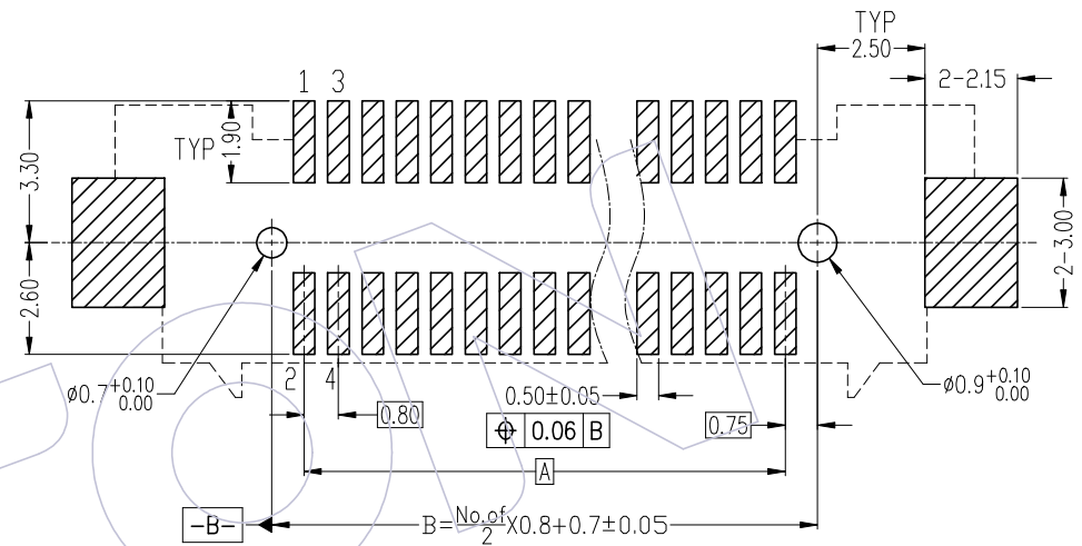
Recommended P.C.B Layout(Top Side) (PCB BOARD TOLERANCE±0.05)
