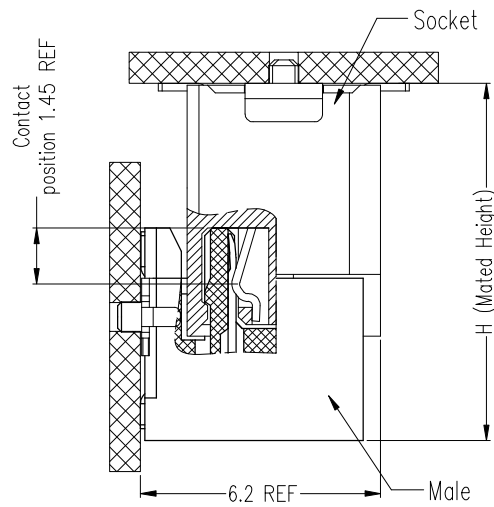
Mated Height diagram
