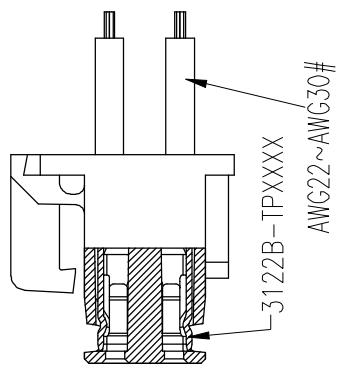
Assembly Hint View
