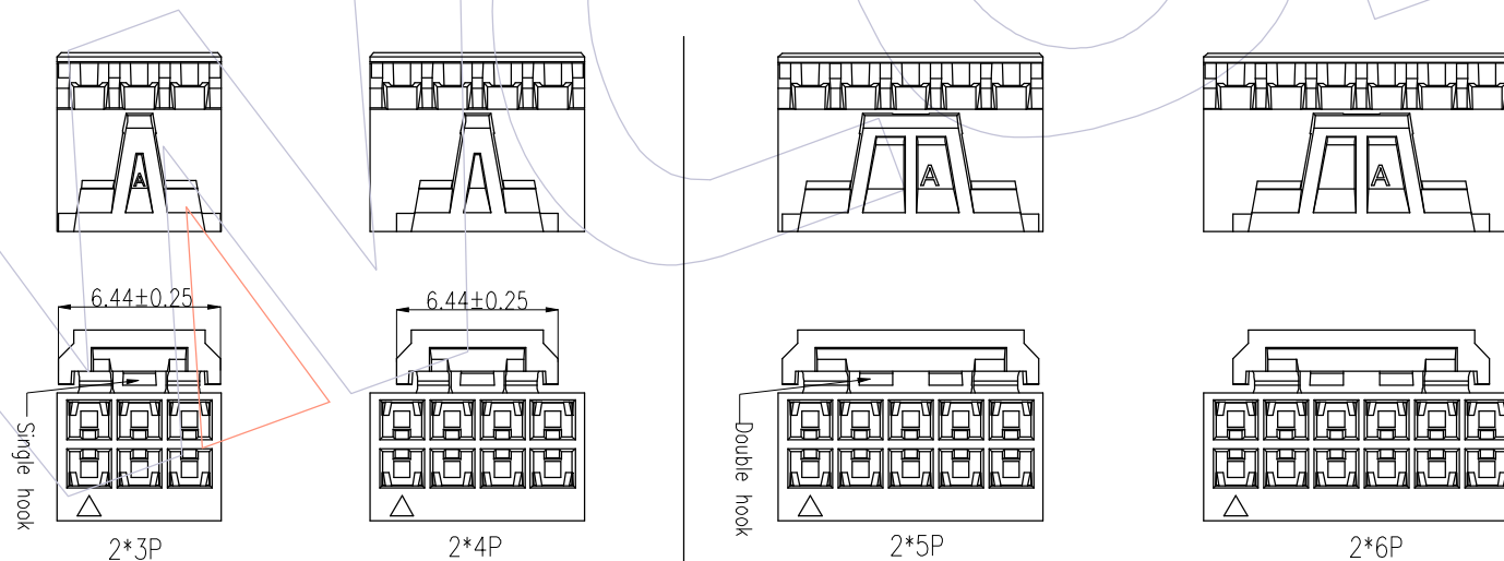
2*3P,2*4P Single hook Configuration
